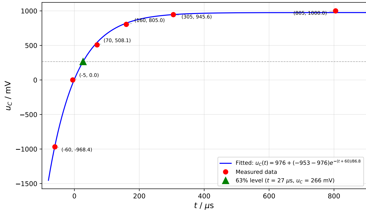
RC Full Response: Exponential Fitting ( \tau = 86.8 \mu\text{s} , R^2 = 0.9983 )
